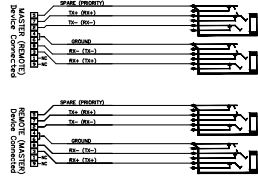
RS422 SCHEMATIC
